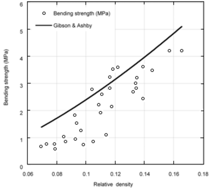
Bending strength vs porosity
